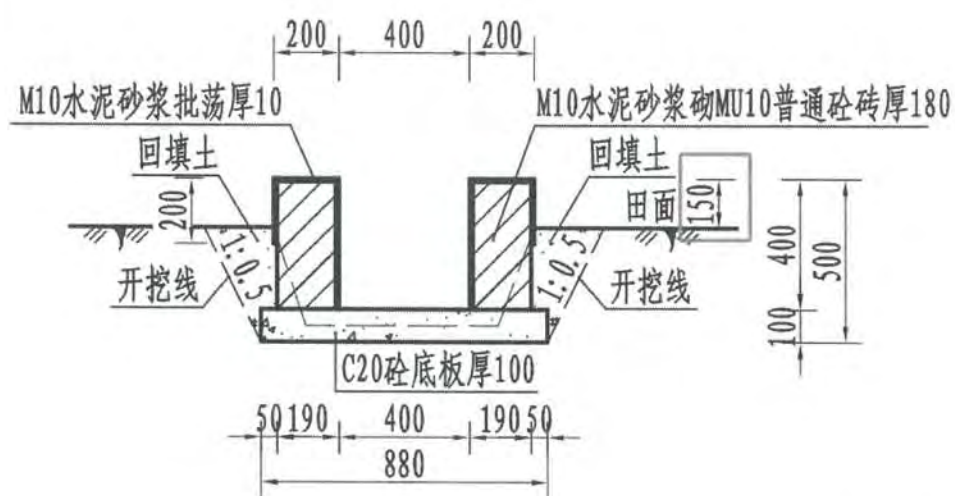
整修农渠IV-3横断面图 1:25 (0.4m×0.4m-80m)
